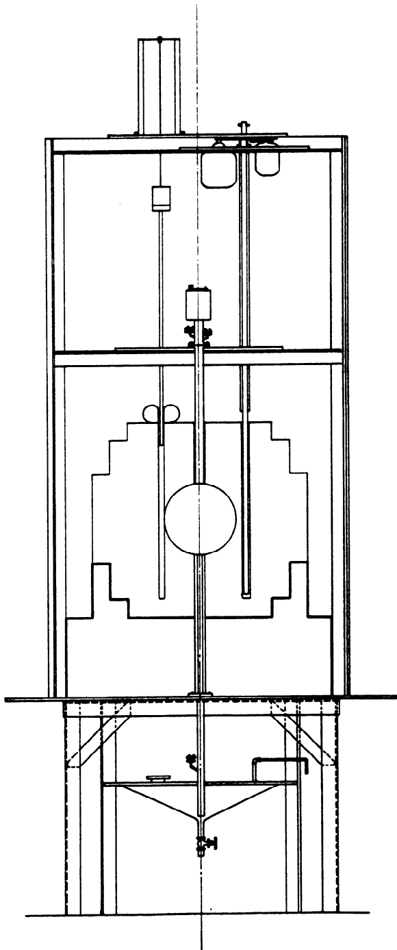
Fig. 1. Schematic of Water Boiler.
