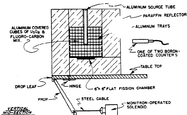
Fig. 4. Cross section of "Drop-Leaf" assembly.
