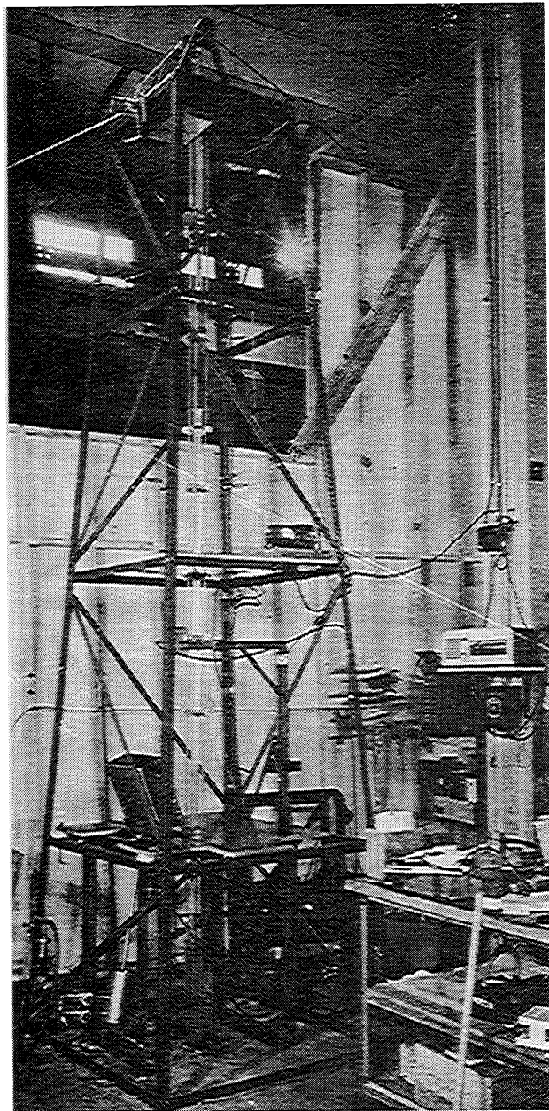
Fig. 3. Derrick framework for Dragon experiment, without active material.
