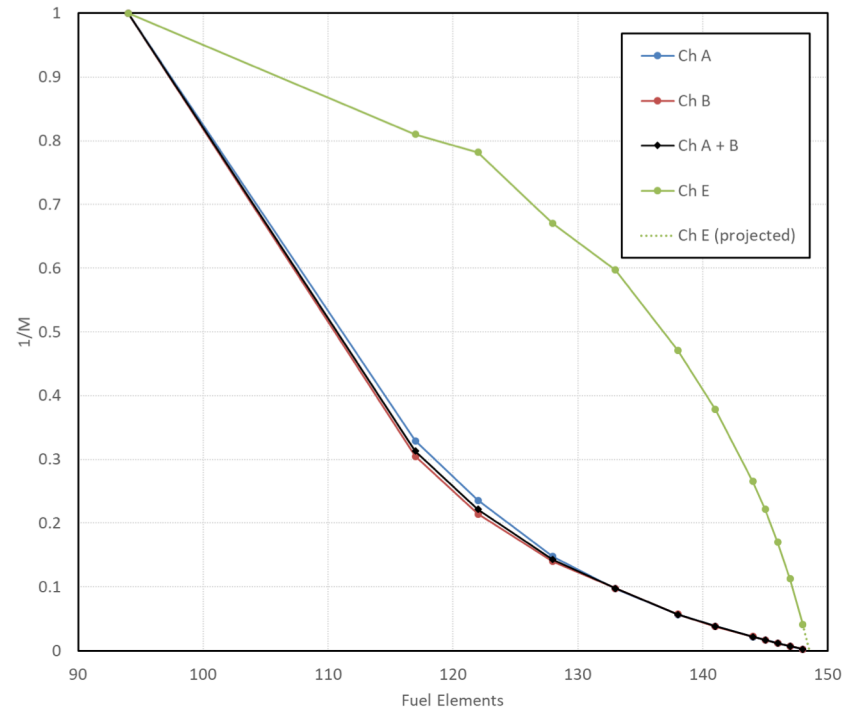
Approach-to-Critical (Case 10)
