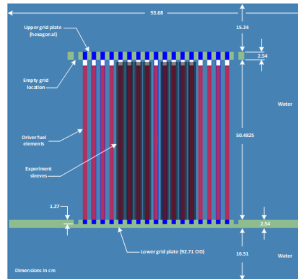
Cut-Away Core
