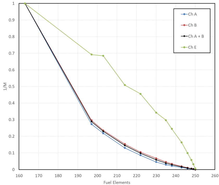
Approach-to-Critical (Case 2)
